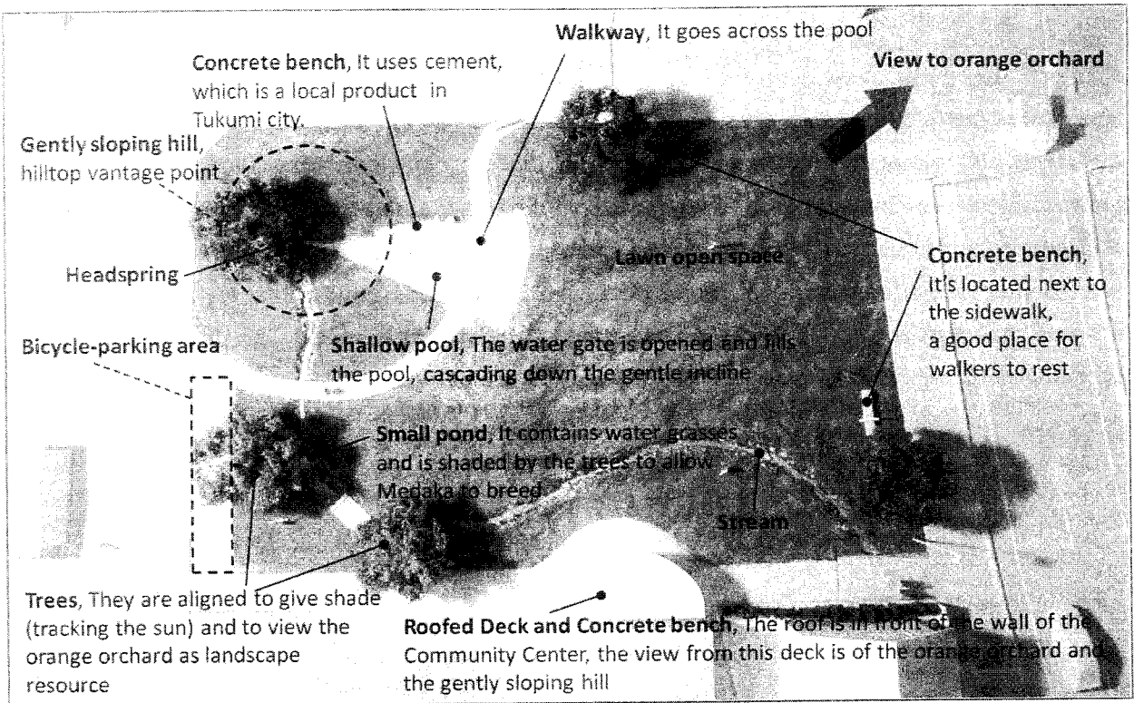
Fig.22 Site plan
