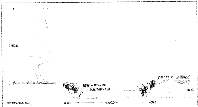
Fig.24 Small pond: section
